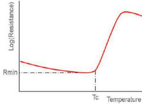
PTC
